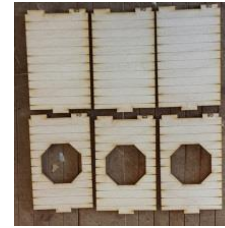
Second floor turret walls C1 thru C6
