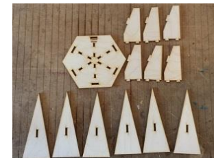
Turret roof assembly
